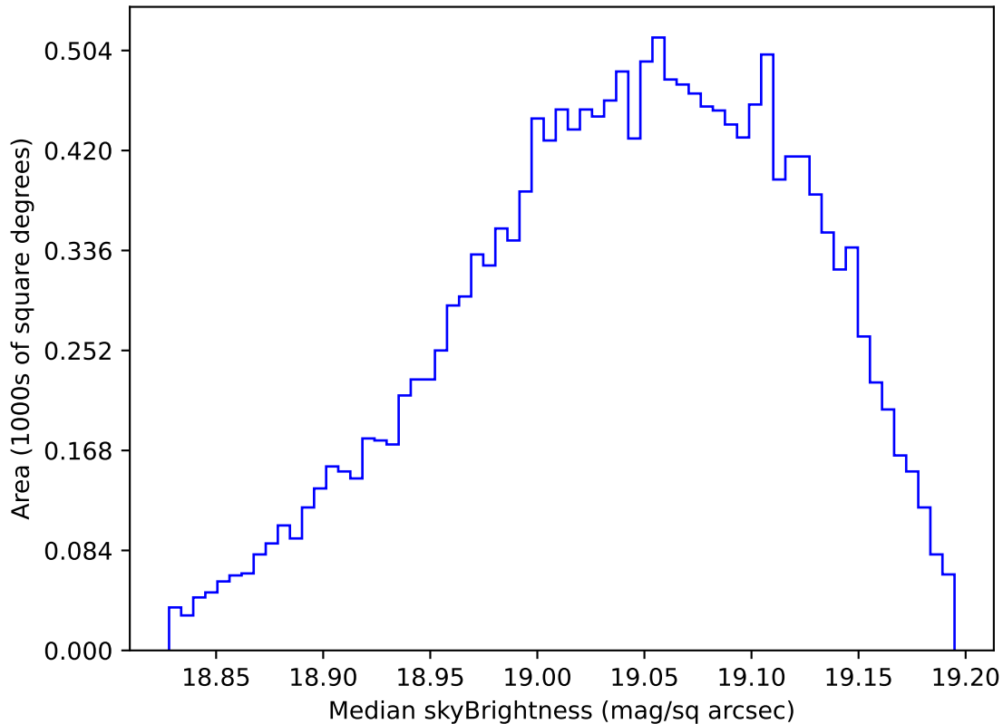
too_elab_heavy_r32_d2_ugrizy_v3.4_10yrs WFD z band: Median skyBrightness
