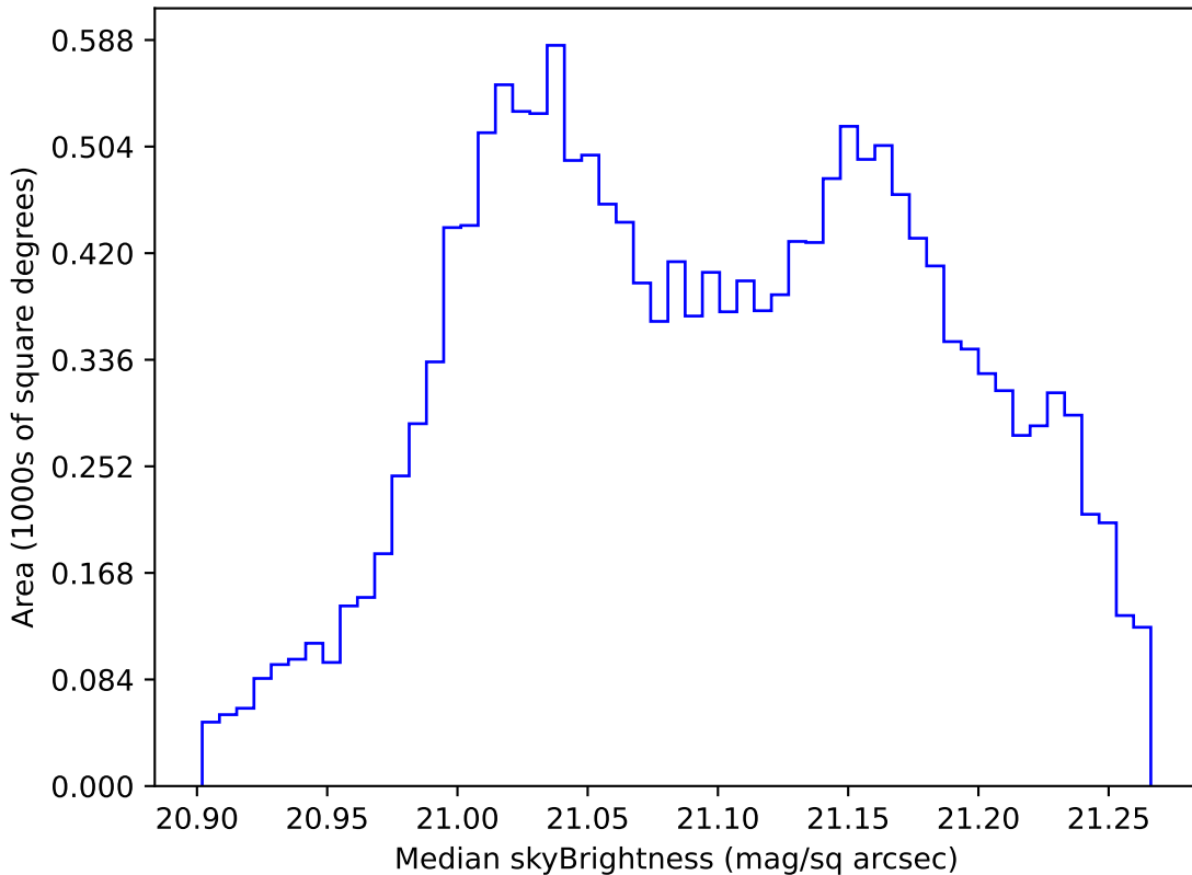
too_elab_heavy_r32_d2_ugrizy_v3.4_10yrs WFD r band: Median skyBrightness
