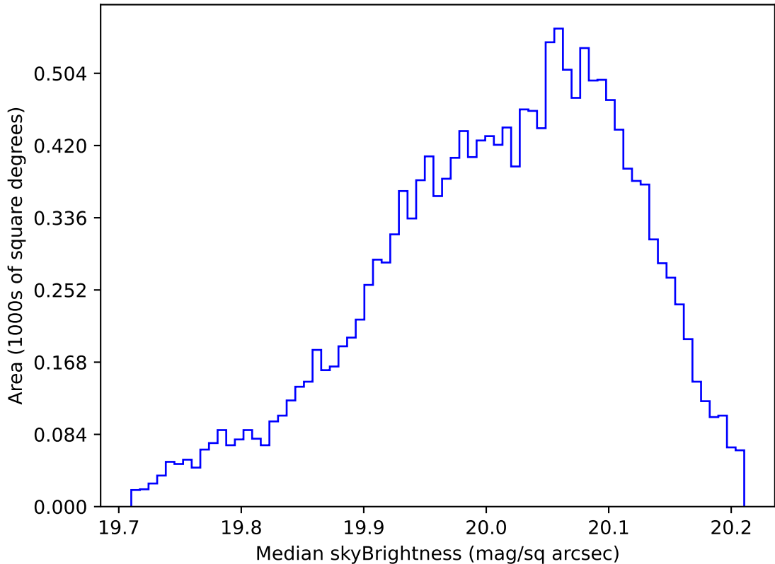
too_elab_heavy_r32_d2_ugrizy_v3.4_10yrs WFD i band: Median skyBrightness
