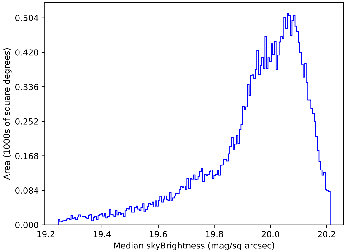
too_elab_heavy_r32_d2_ugrizy_v3.4_10yrs All sky i band: Median skyBrightness
