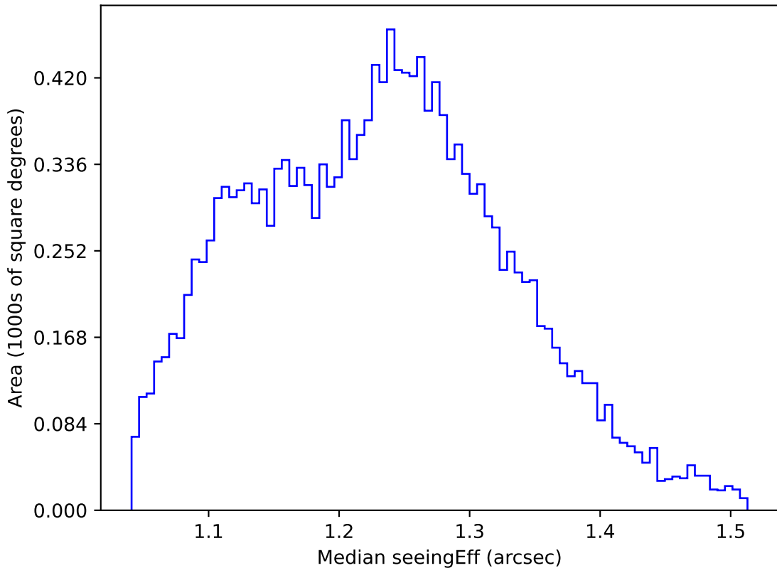
too_elab_heavy_r32_d2_ugrizy_v3.4_10yrs WFD u band: Median seeingEff
