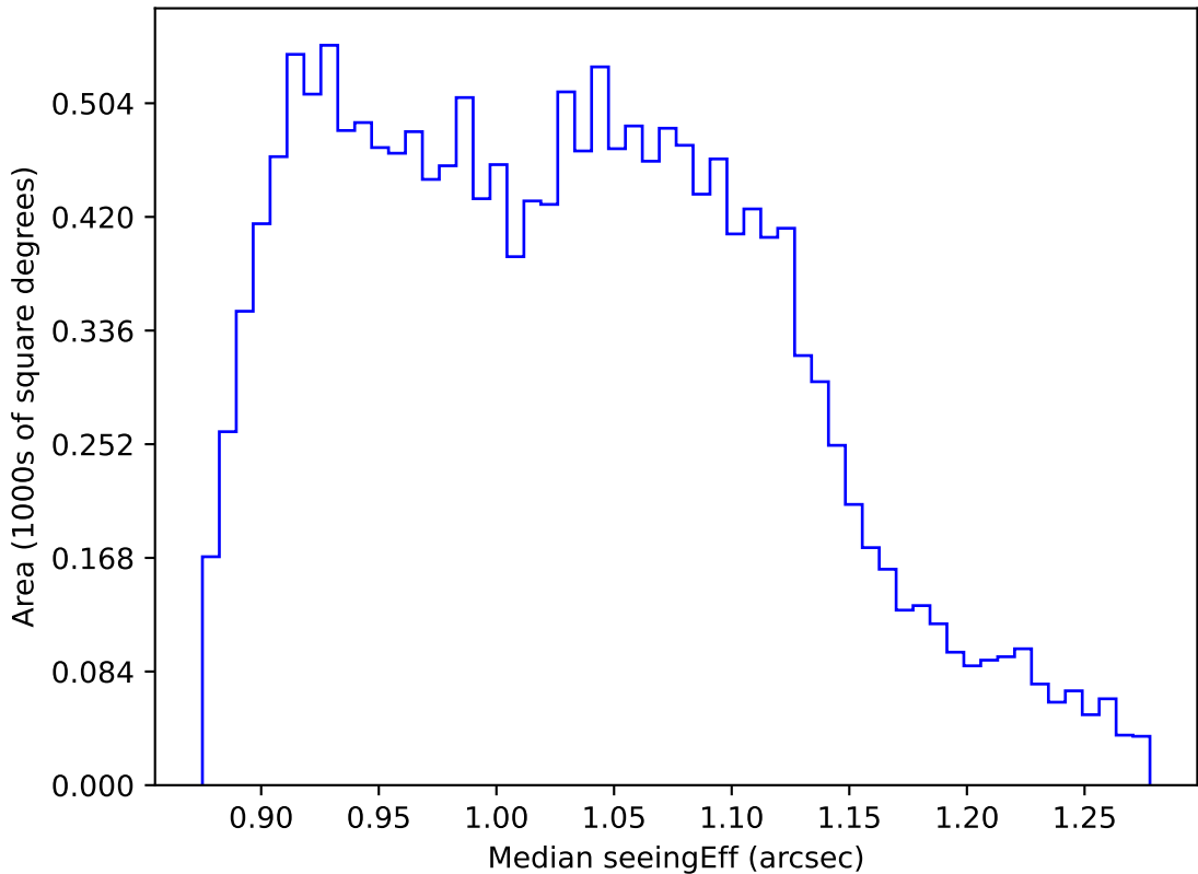
too_elab_heavy_r32_d2_ugrizy_v3.4_10yrs WFD r band: Median seeingEff
