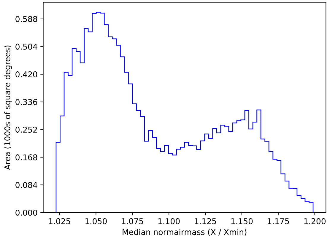
too_elab_heavy_r32_d2_ugrizy_v3.4_10yrs WFD z band: Median normairmass
