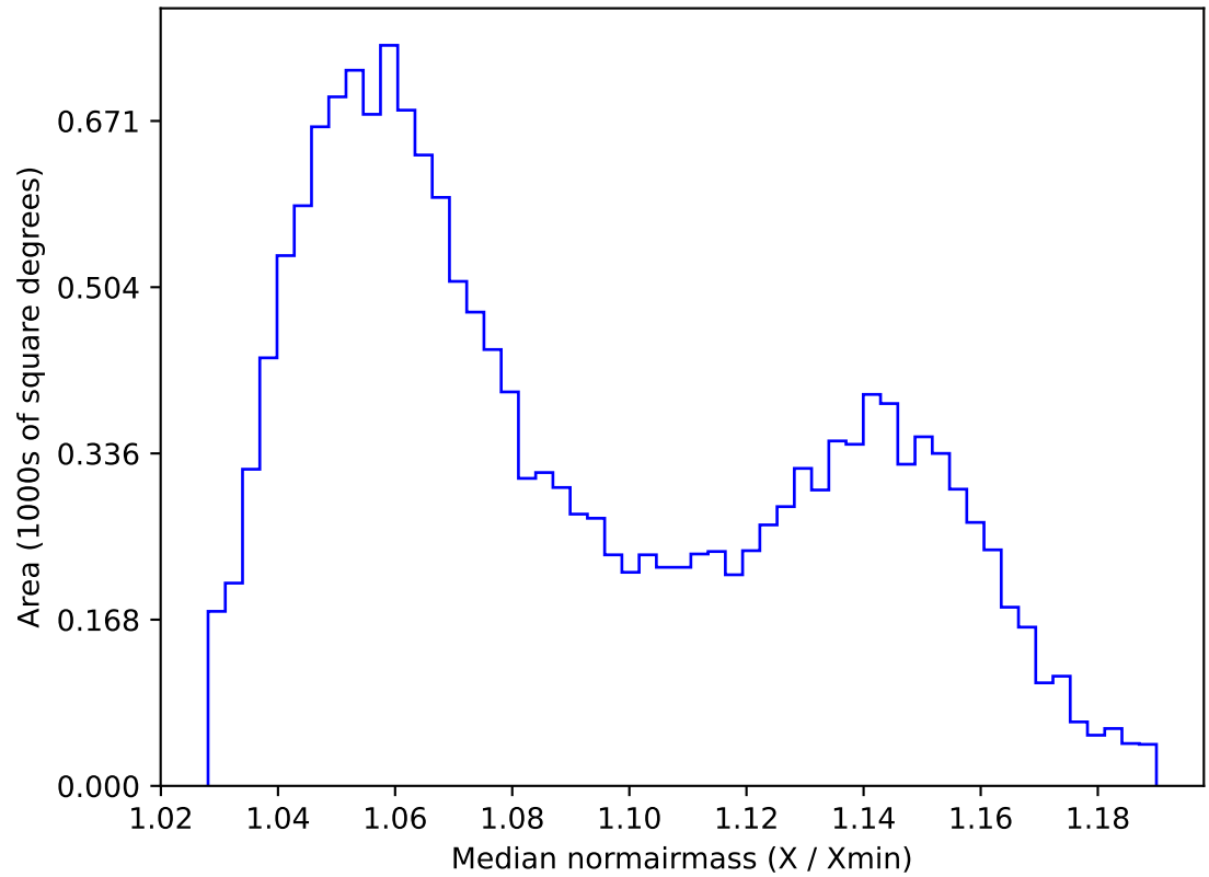
too_elab_heavy_r32_d2_ugrizy_v3.4_10yrs WFD y band: Median normairmass
