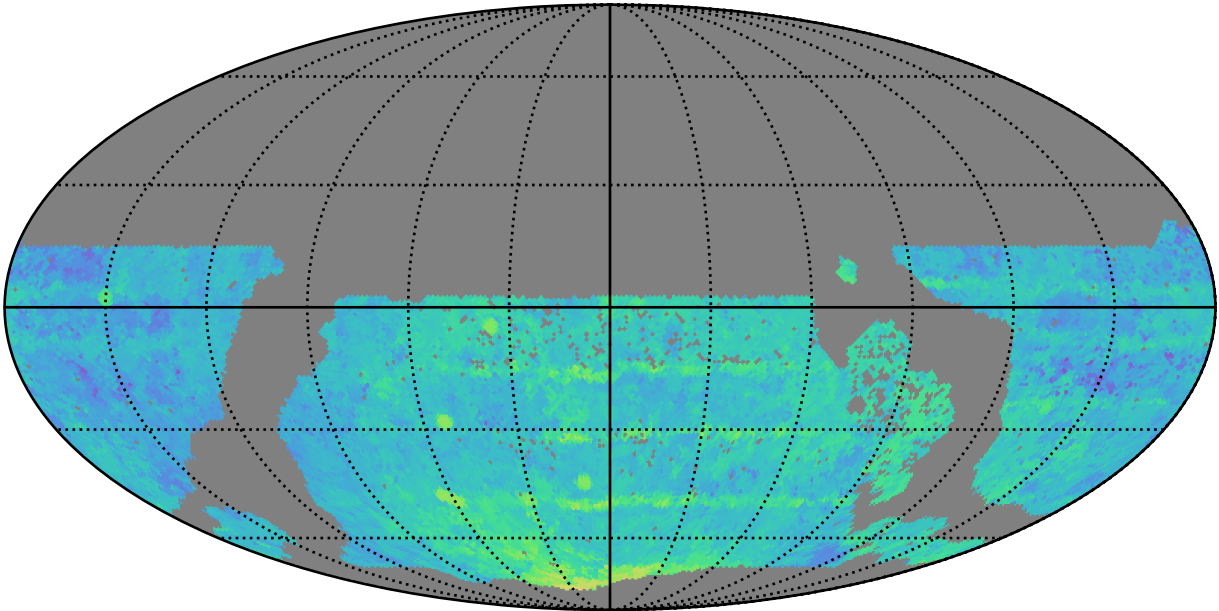
too_elab_heavy_r32_d2_ugrizy_v3.4_10yrs WFD z band: Median Season Length
