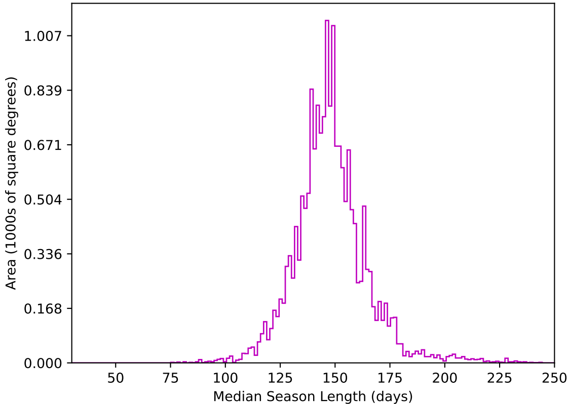
too_elab_heavy_r32_d2_ugrizy_v3.4_10yrs WFD z band: Median Season Length
