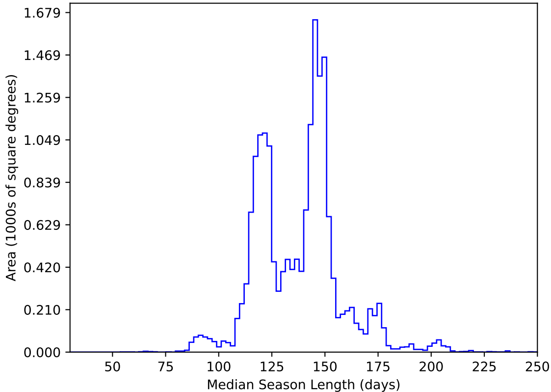
too_elab_heavy_r32_d2_ugrizy_v3.4_10yrs WFD y band: Median Season Length
