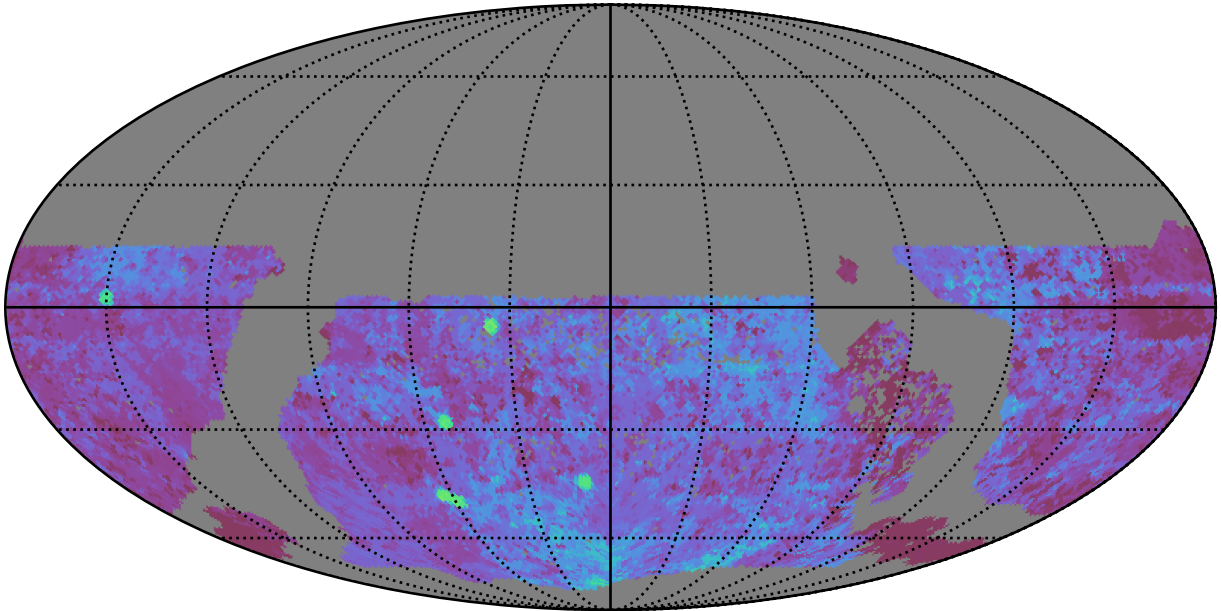
too_elab_heavy_r32_d2_ugrizy_v3.4_10yrs WFD u band: Median Season Length
