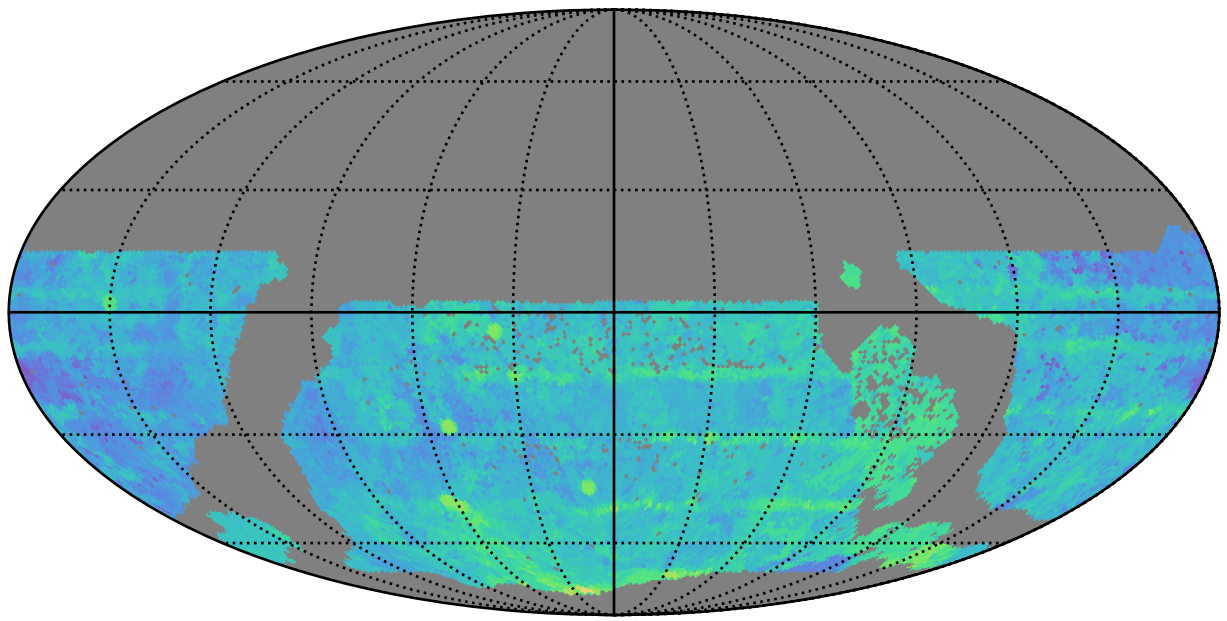
too_elab_heavy_r32_d2_ugrizy_v3.4_10yrs WFD r band: Median Season Length
