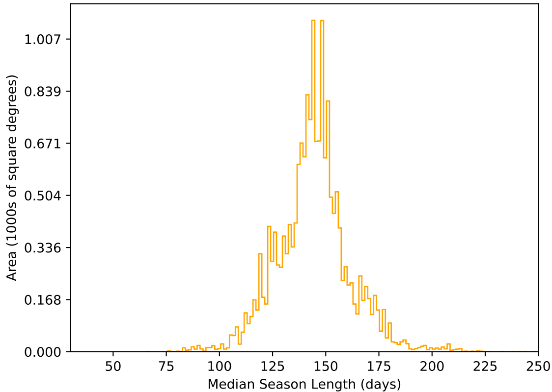
too_elab_heavy_r32_d2_ugrizy_v3.4_10yrs WFD r band: Median Season Length
