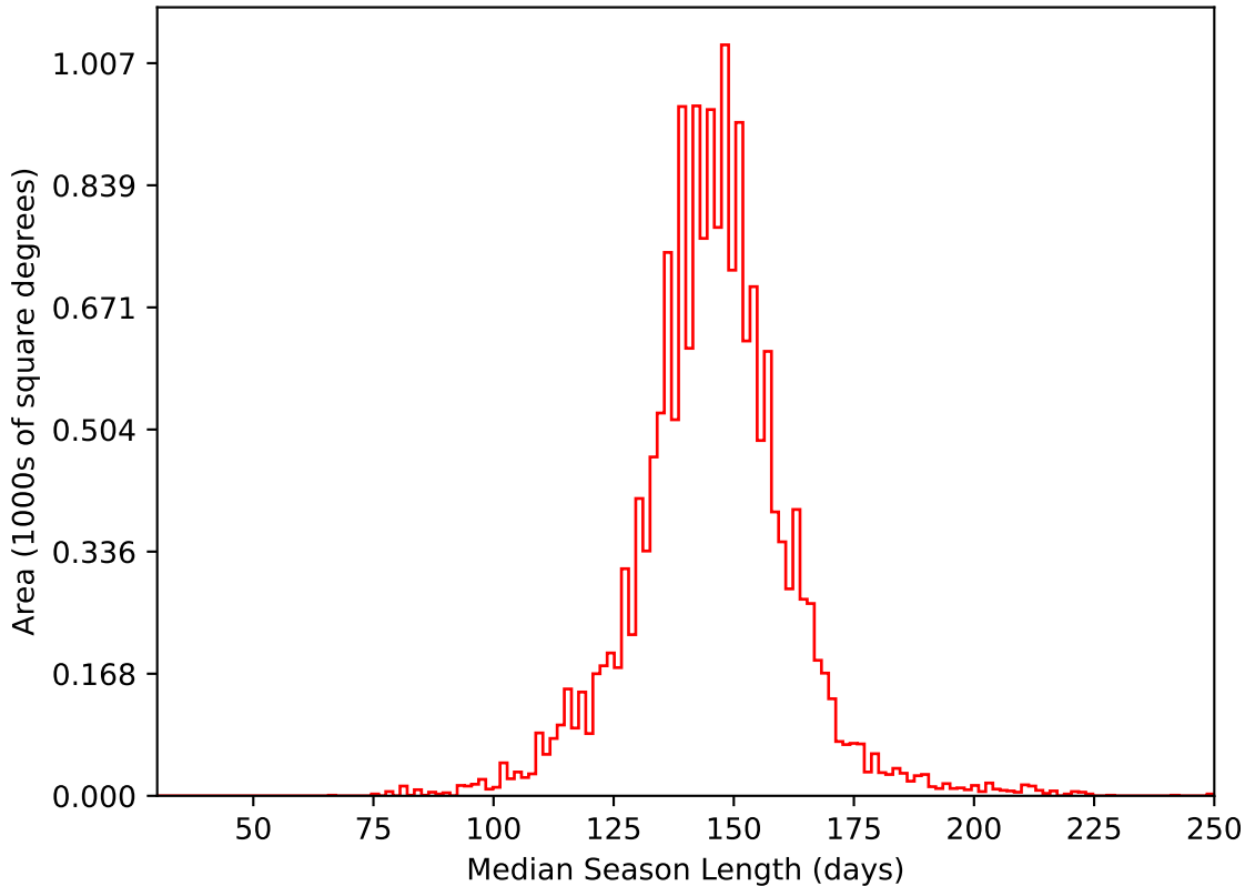
too_elab_heavy_r32_d2_ugrizy_v3.4_10yrs WFD i band: Median Season Length
