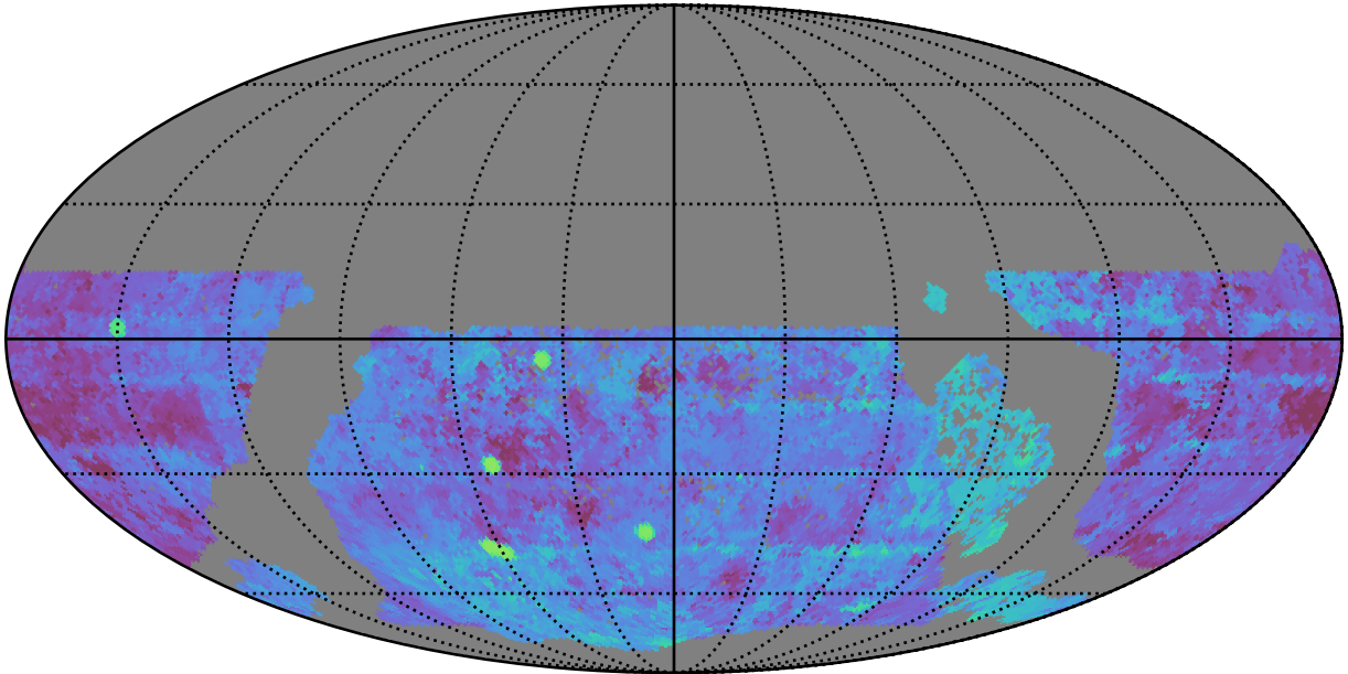
too_elab_heavy_r32_d2_ugrizy_v3.4_10yrs WFD g band: Median Season Length
