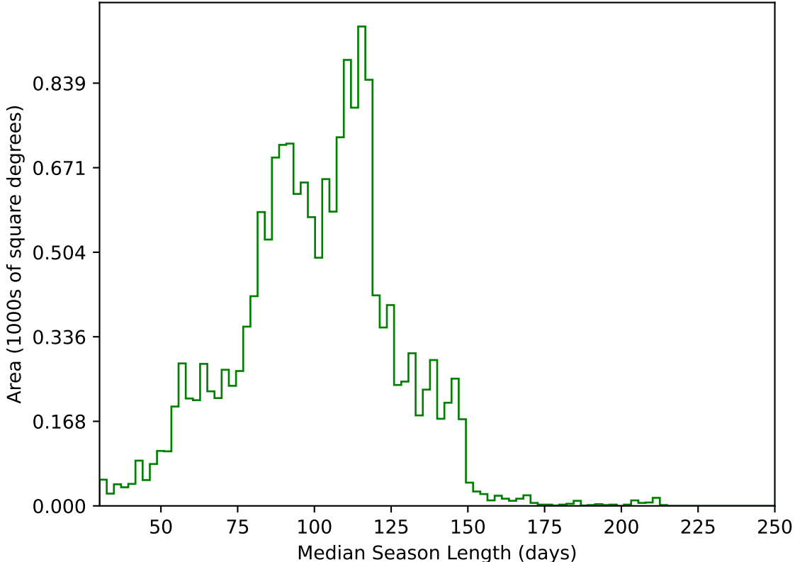
too_elab_heavy_r32_d2_ugrizy_v3.4_10yrs WFD g band: Median Season Length
