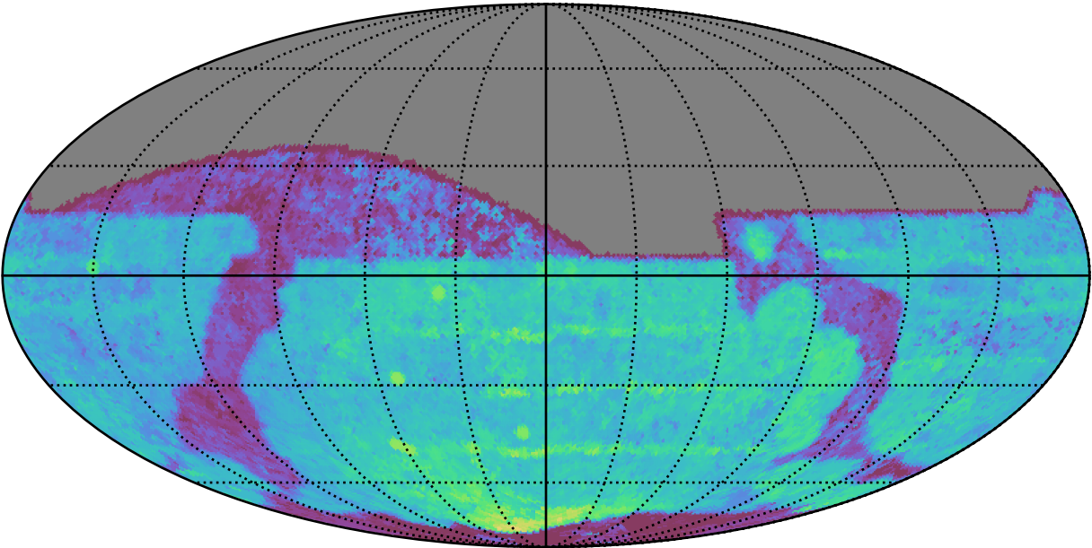
too_elab_heavy_r32_d2_ugrizy_v3.4_10yrs All sky z band: Median Season Length
