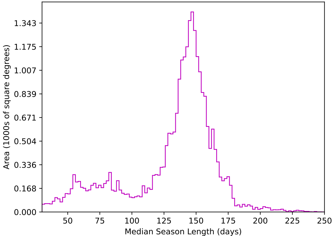
too_elab_heavy_r32_d2_ugrizy_v3.4_10yrs All sky z band: Median Season Length
