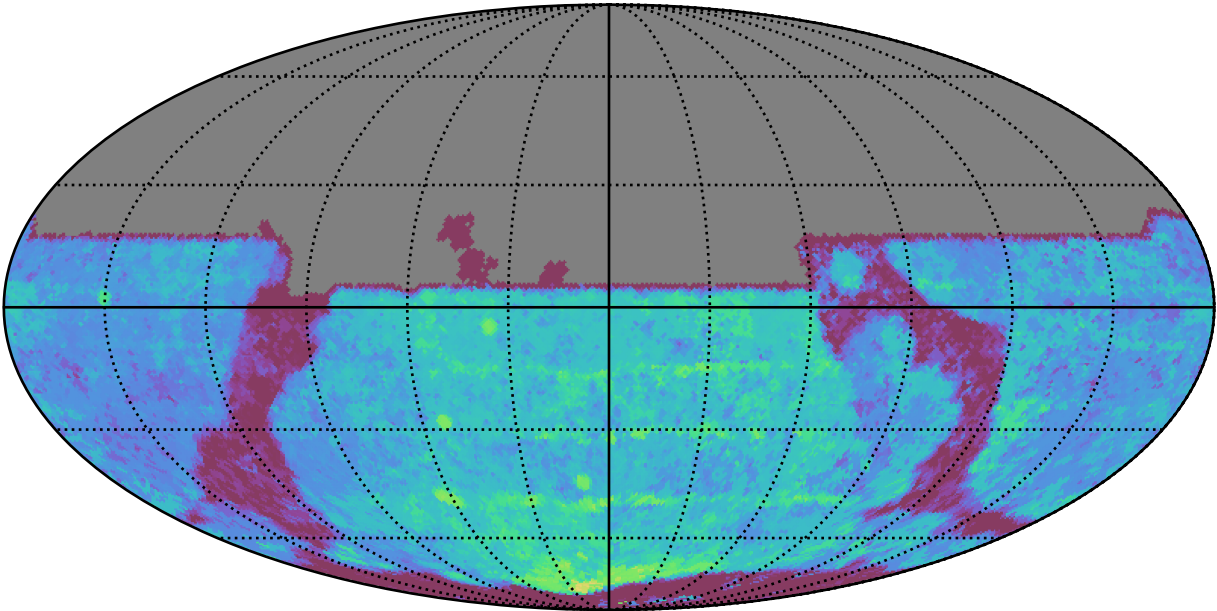
too_elab_heavy_r32_d2_ugrizy_v3.4_10yrs All sky y band: Median Season Length
