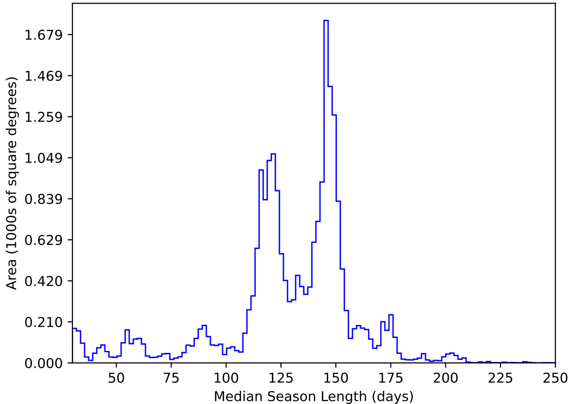
too_elab_heavy_r32_d2_ugrizy_v3.4_10yrs All sky y band: Median Season Length
