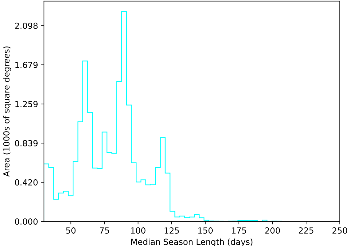
too_elab_heavy_r32_d2_ugrizy_v3.4_10yrs All sky u band: Median Season Length
