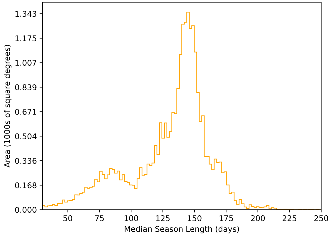
too_elab_heavy_r32_d2_ugrizy_v3.4_10yrs All sky r band: Median Season Length
