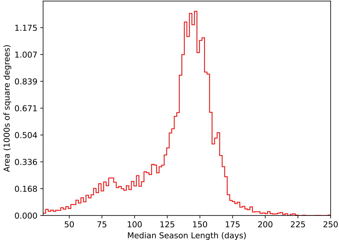
too_elab_heavy_r32_d2_ugrizy_v3.4_10yrs All sky i band: Median Season Length
