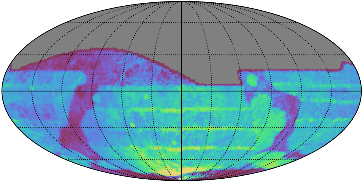
too_elab_heavy_r32_d2_ugrizy_v3.4_10yrs All sky all bands: Median Season Length
