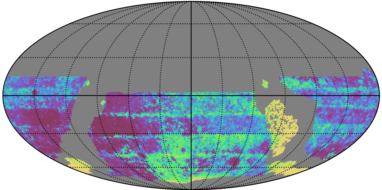
too_elab_heavy_r32_d2_ugrizy_v3.4_10yrs WFD y band: Median Inter-Night Gap
