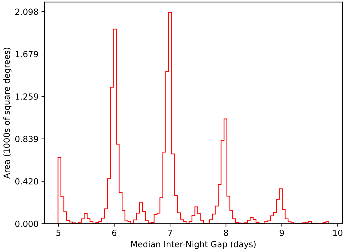
too_elab_heavy_r32_d2_ugrizy_v3.4_10yrs WFD i band: Median Inter-Night Gap
