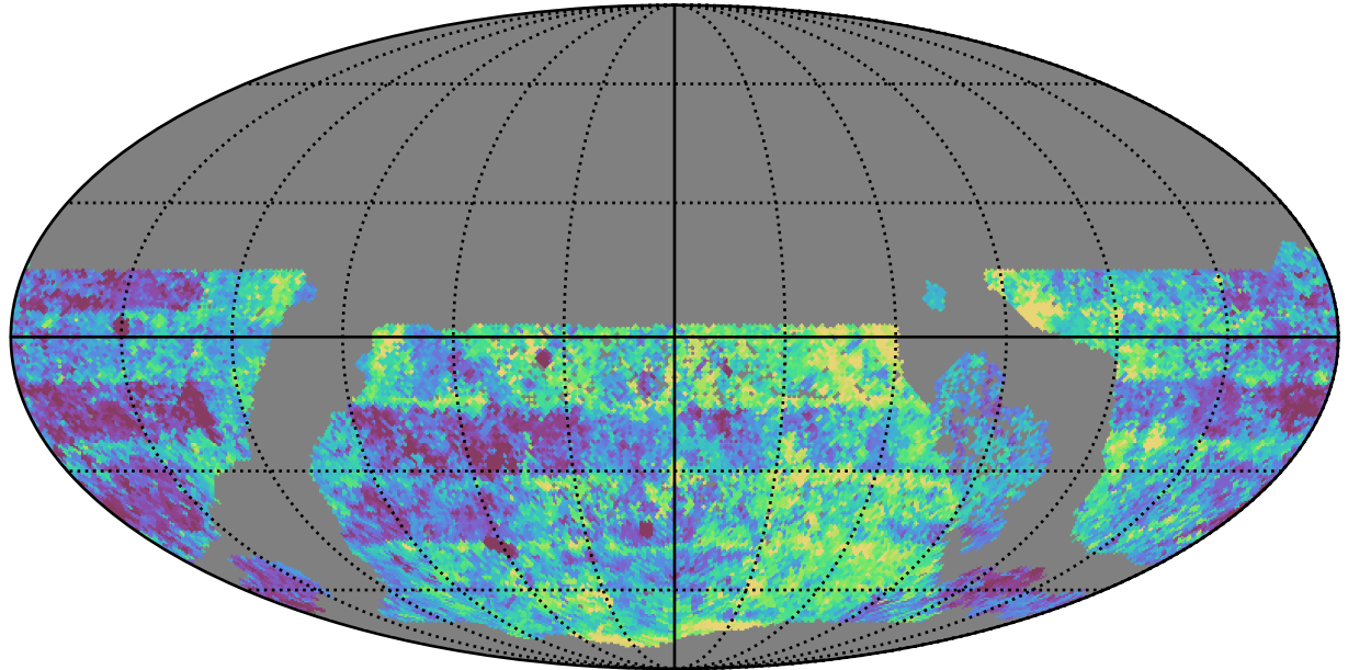
too_elab_heavy_r32_d2_ugrizy_v3.4_10yrs WFD g band: Median Inter-Night Gap
