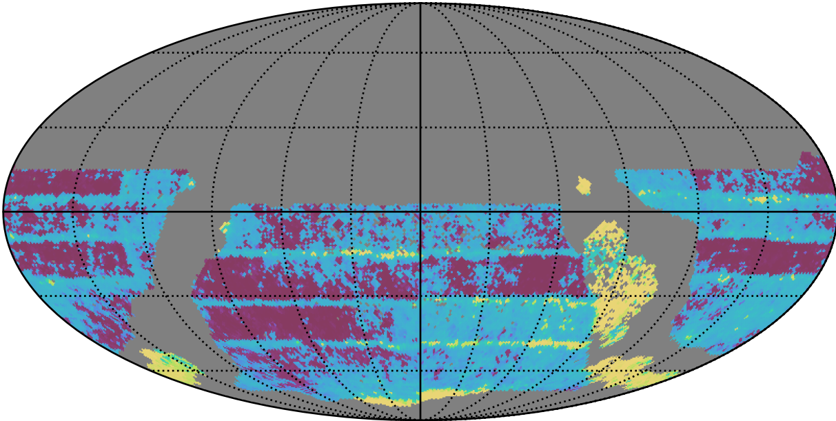
too_elab_heavy_r32_d2_ugrizy_v3.4_10yrs WFD all bands: Median Inter-Night Gap
