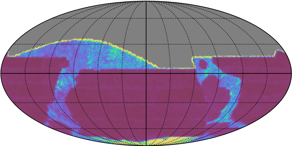
too_elab_heavy_r32_d2_ugrizy_v3.4_10yrs All sky i band: Median Inter-Night Gap
