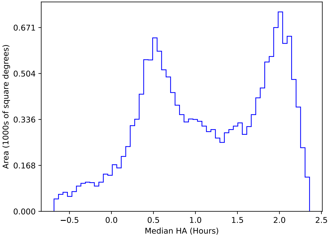
too_elab_heavy_r32_d2_ugrizyv3.4_10yrs WFD z band: Median HA
