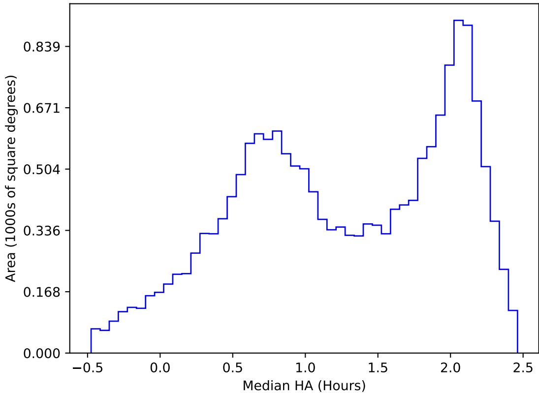
too_elab_heavy_r32_d2_ugrizy_v3.4_10yrs WFD y band: Median HA
