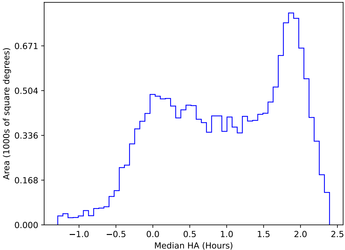
too_elab_heavy_r32_d2_ugrizy_v3.4_10yrs WFD u band: Median HA
