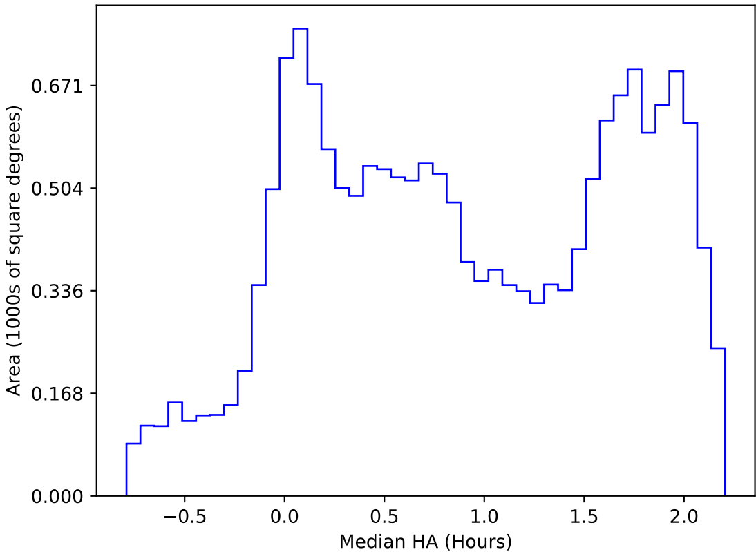
too_elab_heavy_r32_d2_ugrizy_v3.4_10yrs WFD r band: Median HA
