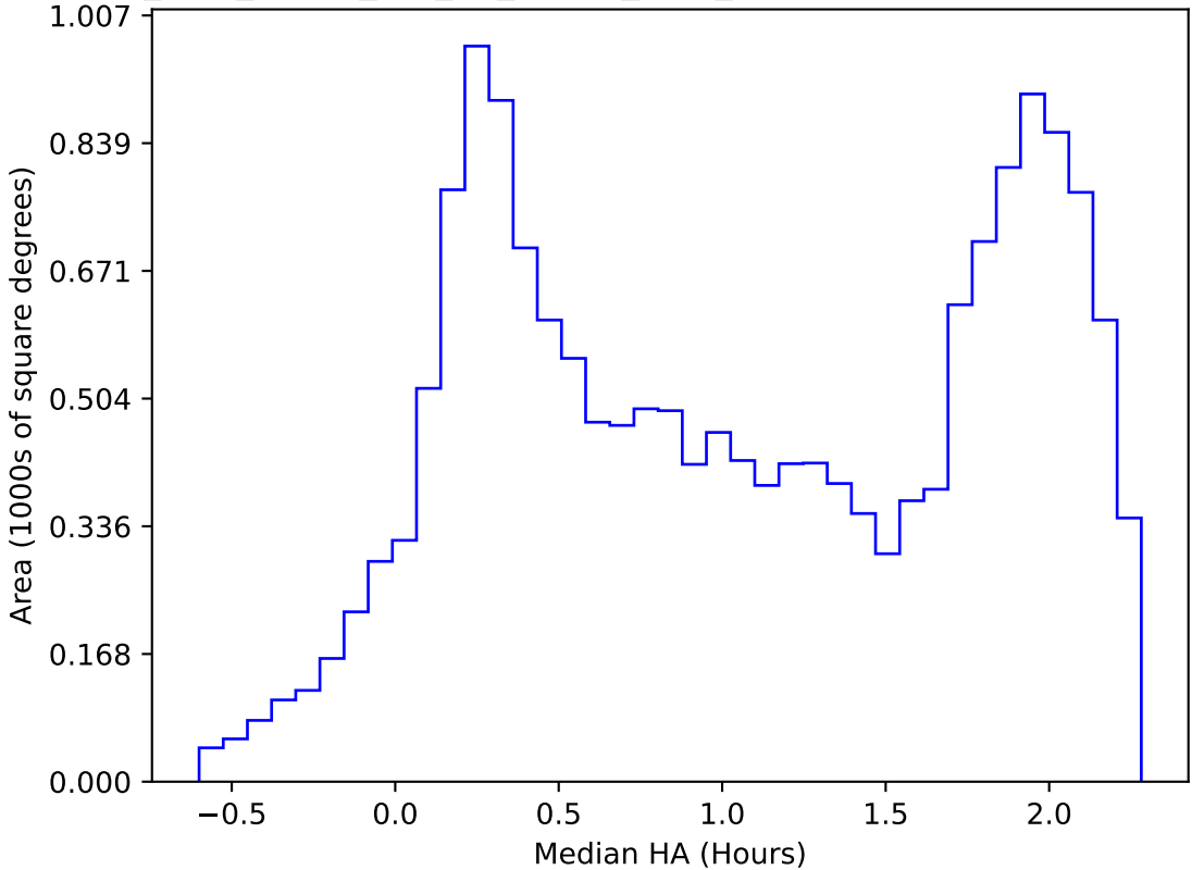
too_elab_heavy_r32_d2_ugrizy_v3.4_10yrs WFD i band: Median HA
