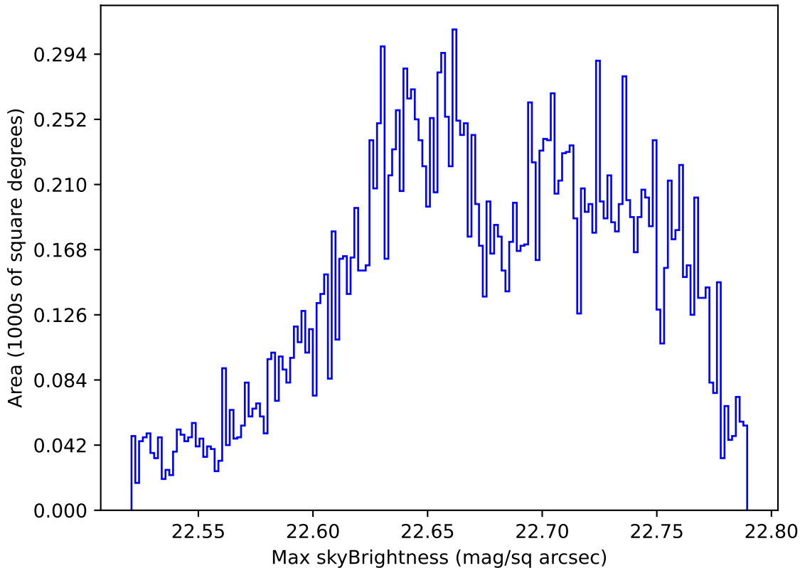
too_elab_heavy_r32_d2_ugrizy_v3.4_10yrs Yr 1 u band: Max skyBrightness
