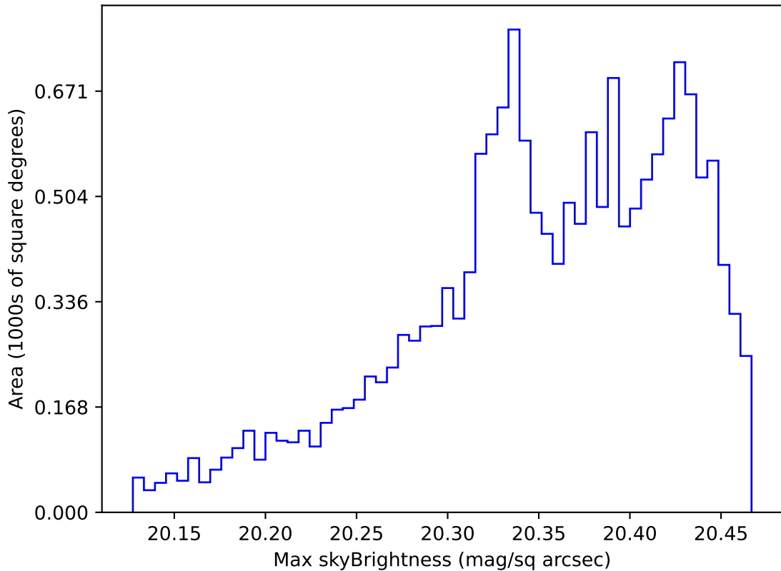
too_elab_heavy_r32_d2_ugrizy_v3.4_10yrs WFD i band: Max skyBrightness
