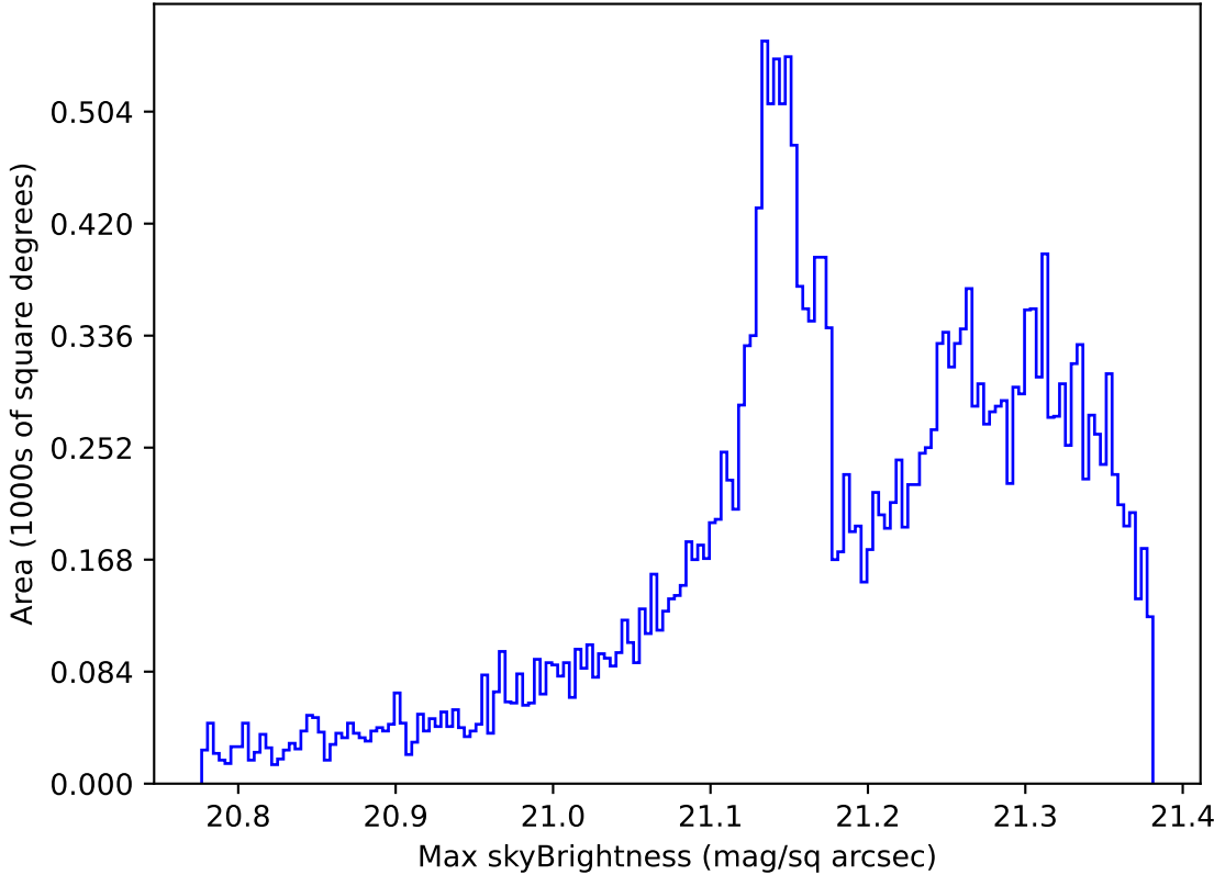
too_elab_heavy_r32_d2_ugrizy_v3.4_10yrs All sky r band: Max skyBrightness
