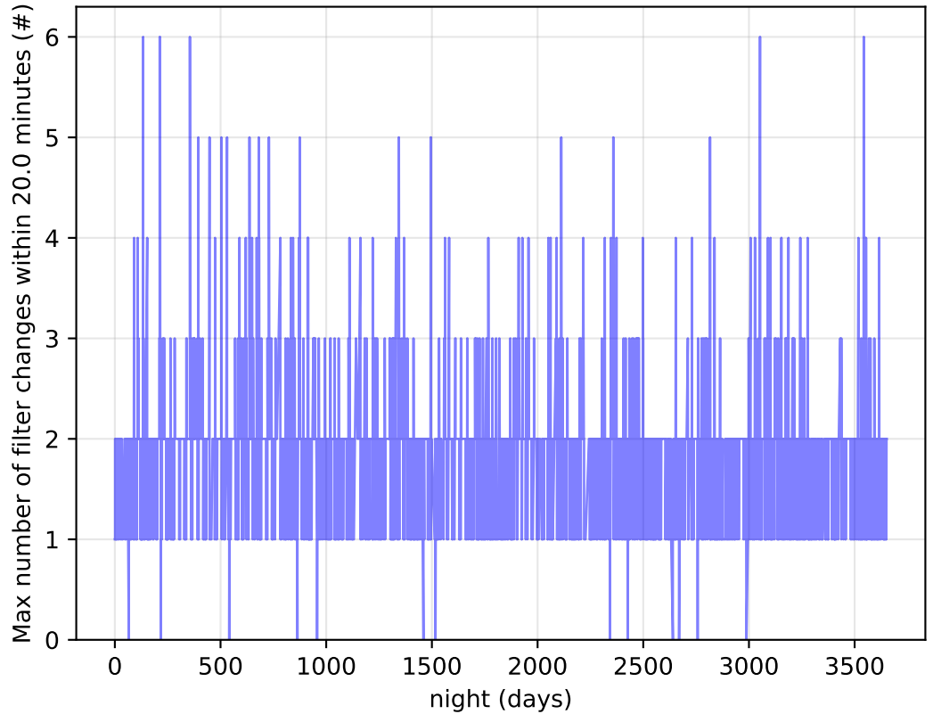
too_elab_heavy_r32_d2_ugrizy_v3.4_10yrs Per Night: Max number of filter changes within 20.0 minutes
