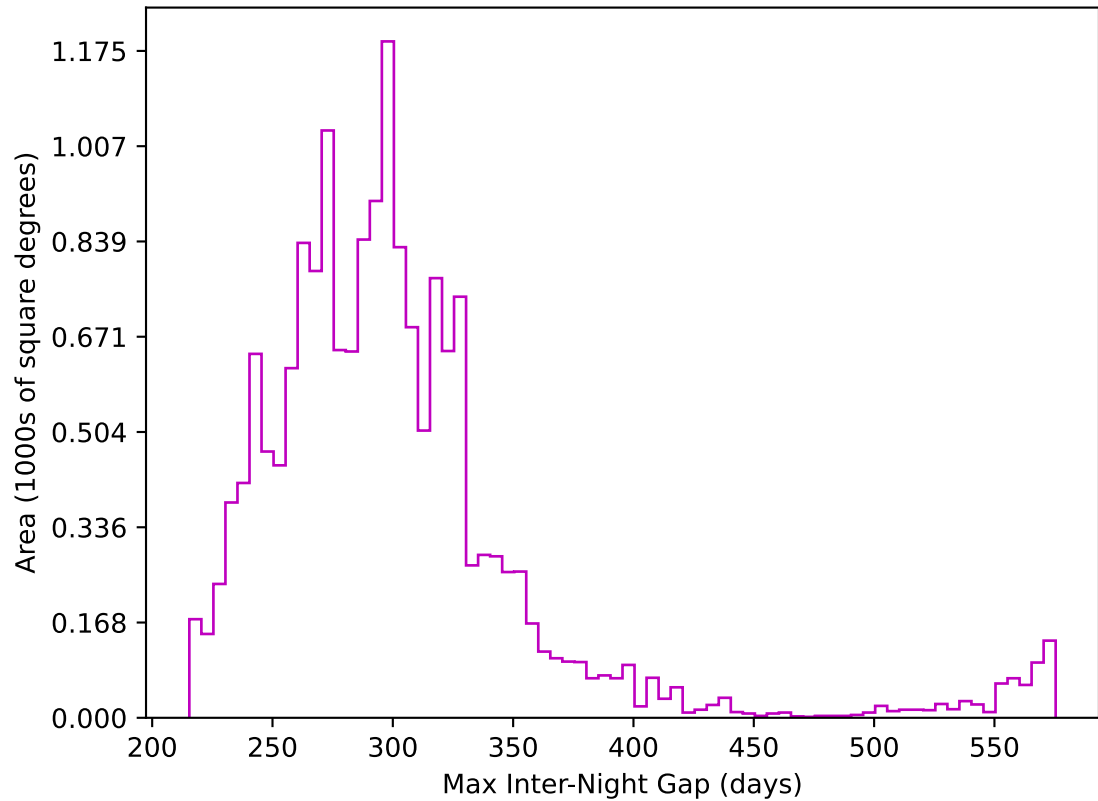
too_elab_heavy_r32_d2_ugrizy_v3.4_10yrs WFD z band: Max Inter-Night Gap
