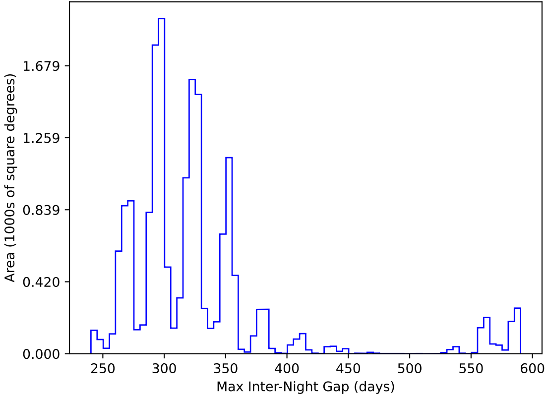
too_elab_heavy_r32_d2_ugrizy_v3.4_10yrs WFD y band: Max Inter-Night Gap
