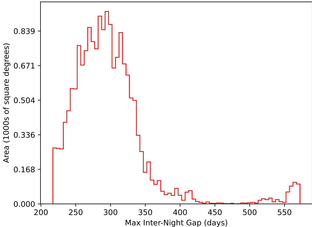
too_elab_heavy_r32_d2_ugrizy_v3.4_10yrs WFD i band: Max Inter-Night Gap
