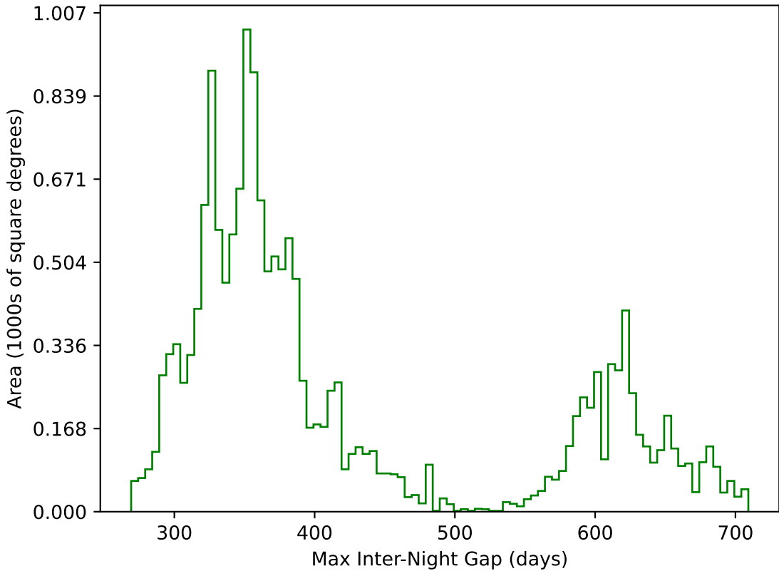
too_elab_heavy_r32_d2_ugrizy_v3.4_10yrs WFD g band: Max Inter-Night Gap
