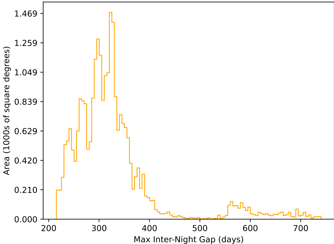
too_elab_heavy_r32_d2_ugrizy_v3.4_10yrs All sky r band: Max Inter-Night Gap
