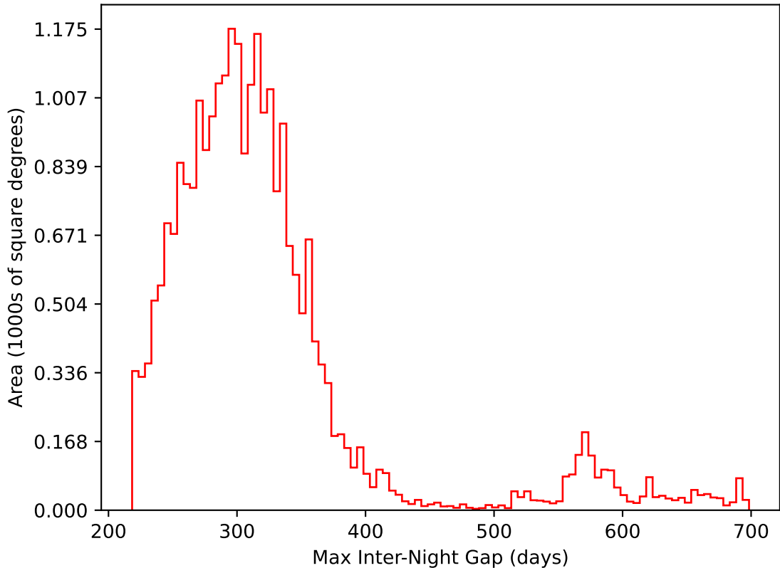
too_elab_heavy_r32_d2_ugrizy_v3.4_10yrs All sky i band: Max Inter-Night Gap
