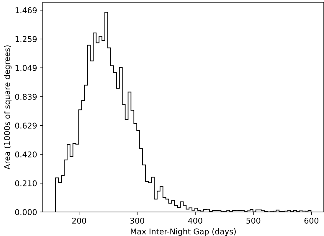
too_elab_heavy_r32_d2_ugrizy_v3.4_10yrs All sky all bands: Max Inter-Night Gap
