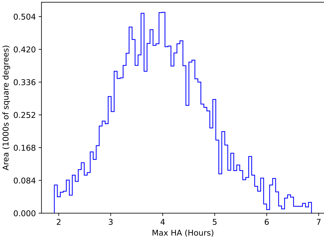
too_elab_heavy_r32_d2_ugrizy_v3.4_10yrs WFD u band: Max HA
