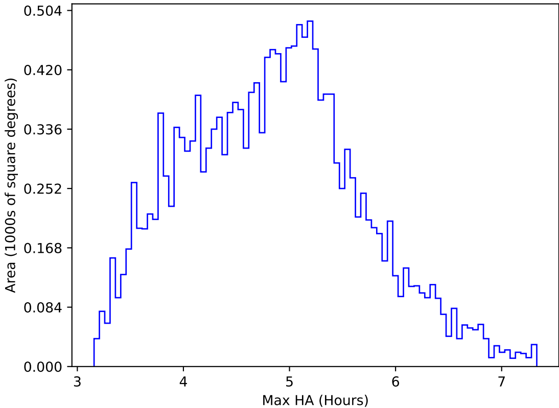
too_elab_heavy_r32_d2_ugrizy_v3.4_10yrs WFD i band: Max HA
