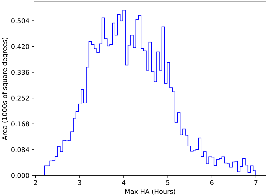
too_elab_heavy_r32_d2_ugrizy_v3.4_10yrs WFD g band: Max HA
