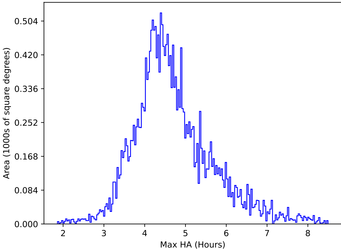
too_elab_heavy_r32_d2_ugrizy_v3.4_10yrs All sky y band: Max HA
